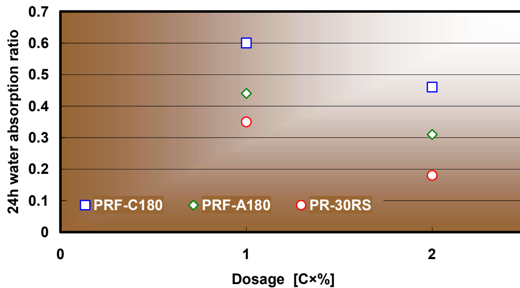
Figure 14. Relationship between waterproofing agents dosage and 24h water absorption ratio.
